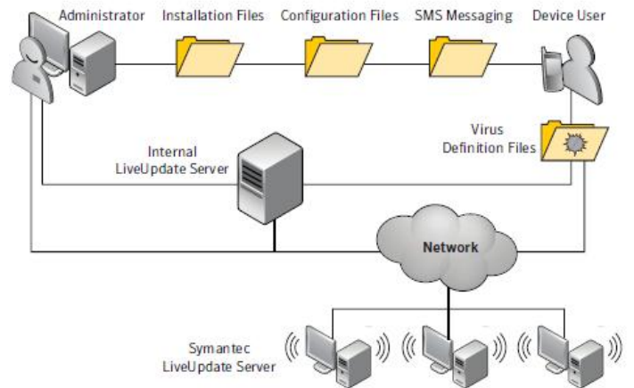
Figure 1. Management and updating of Symantec Mobile Security for Symbian
