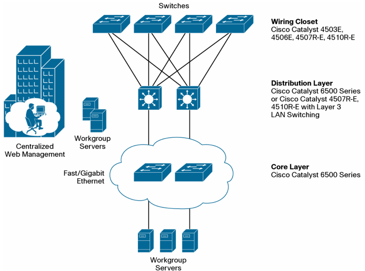
Figure 2. Large Enterprise Network with Cisco Catalyst 4500 Series Switches
