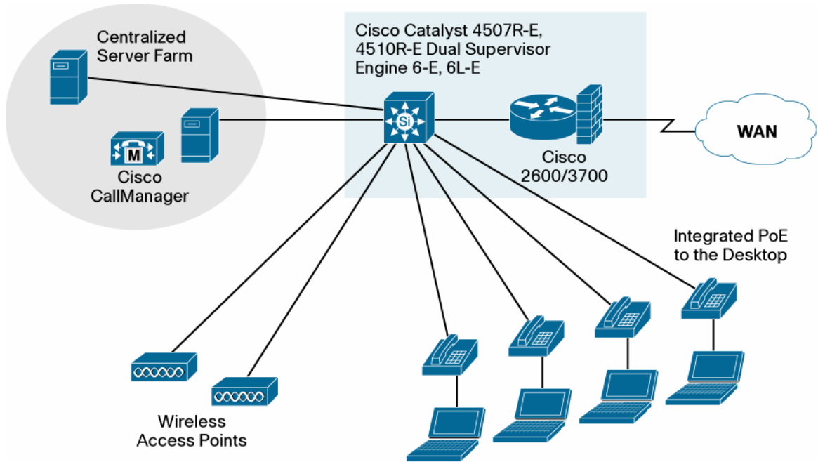
Figure 4. Small-Enterprise and Branch-Office Applications
