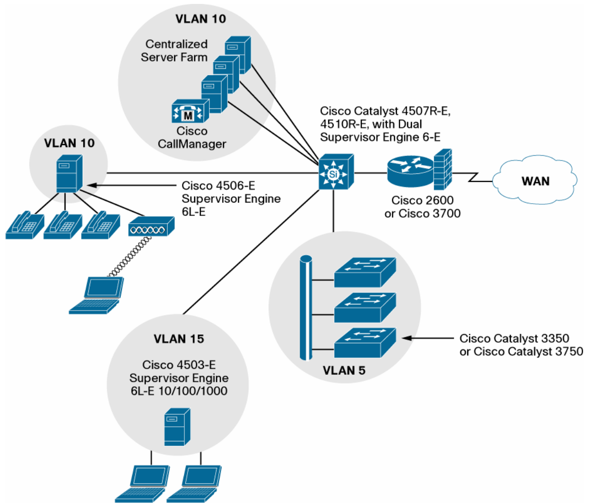
Figure 3. Cisco Catalyst Solution for Medium-Sized Enterprise
